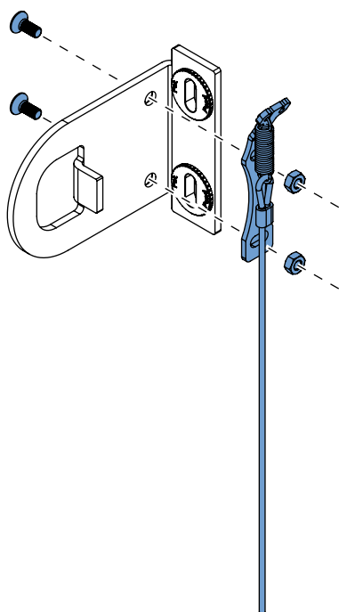
Wall mounting
