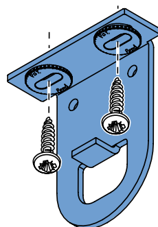
Ceiling mounting
